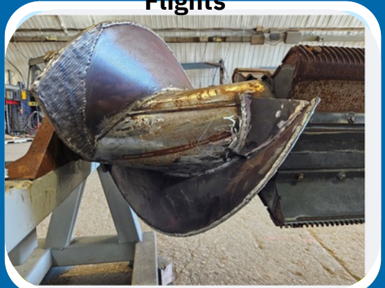
Conversion To Two Aggressive Flights
